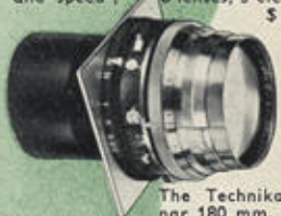
Technika Biogon 53 mm. f/4.5; LINHOF EXCLUSIVE; extreme wide-angle lens of exceptional quality and 'speed'. 8 lenses, 5 elements. $ 436.00
